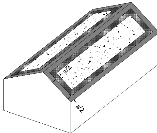
Roof Pitch \geq 10^\circ
