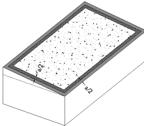
Mono-Slope Roof >math>> 10^\circ</math>
