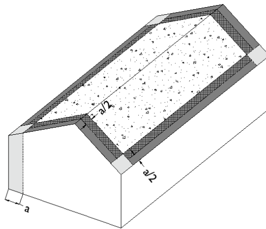
Roof Pitch <math>< 10^\circ</math>
