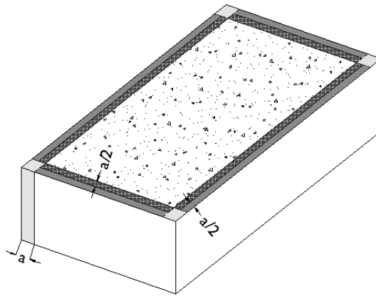
Flat/ Mono-Slope Roof <math>< 10^\circ</math>
